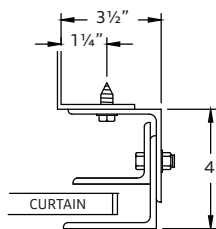
3 piece Structural Steel Guide
